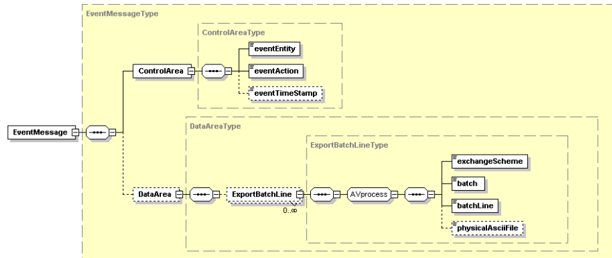
Figure 3-2: XSD for end of set event
