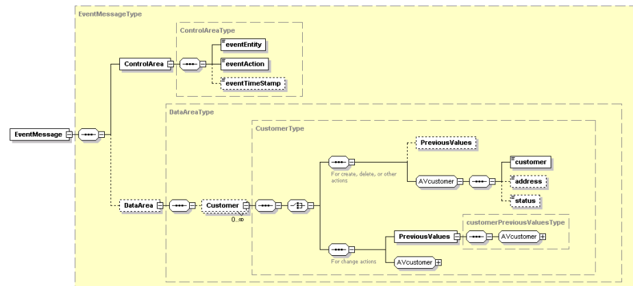
Figure 3-1: XSD for change event
