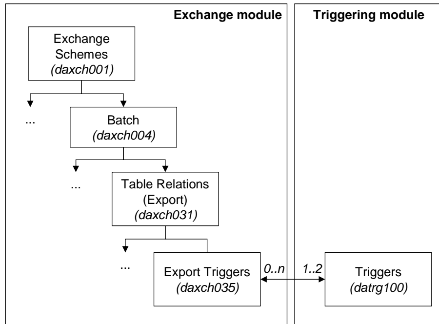
Figure B-1: Export triggers and their context
