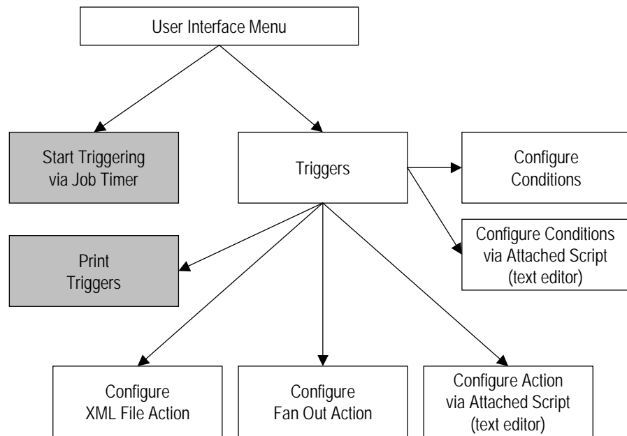
Figure A-1: User interface structure
